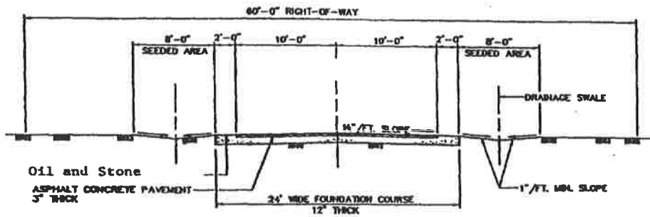
TYPICAL SECTION - ASPHALT CONCRETE PAVEMENT
