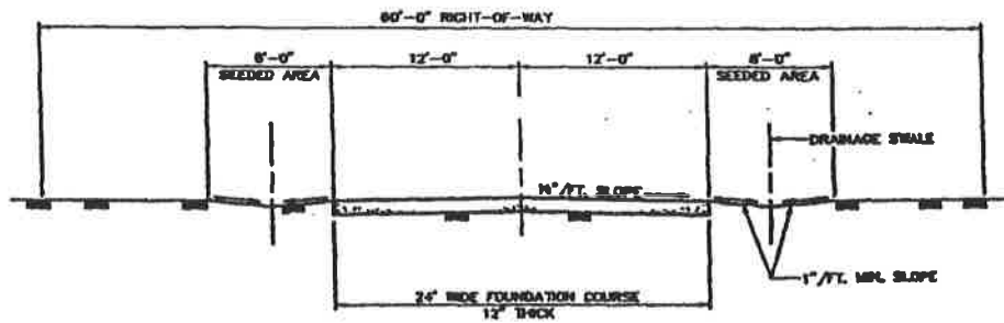
TYPICAL SECTION - OIL AND STONE
